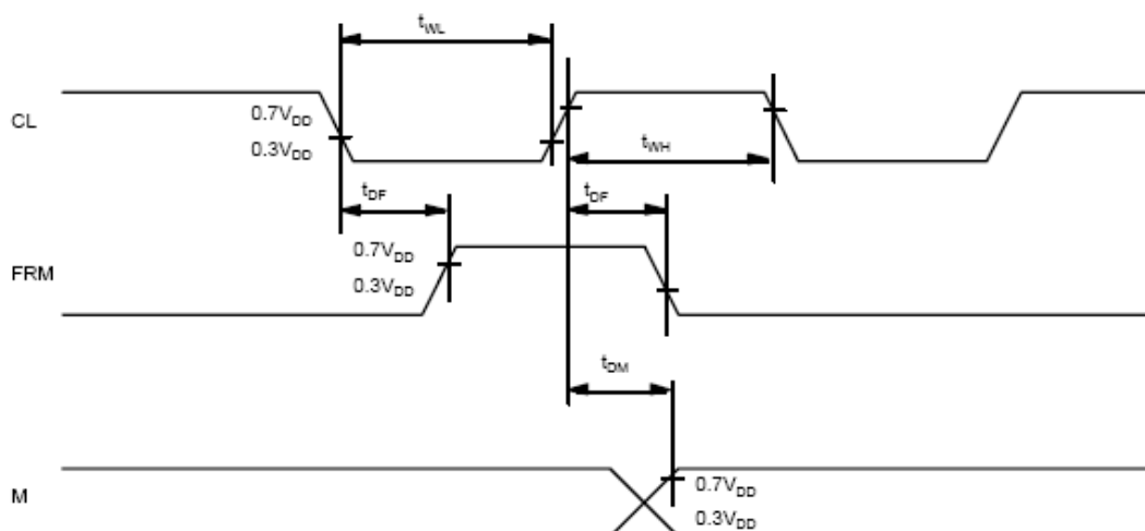
Figure 2. Display control signal waveform
