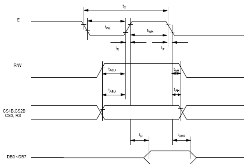
Figure 4. MPU Read Timing
