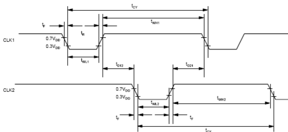
Figure 1. External clock waveform
