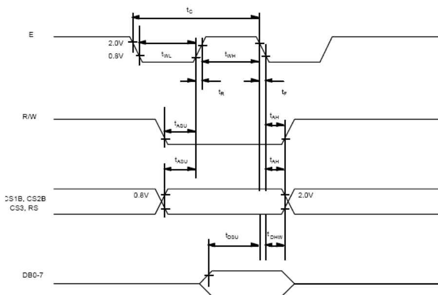
Figure 3. MPU Write Timing
