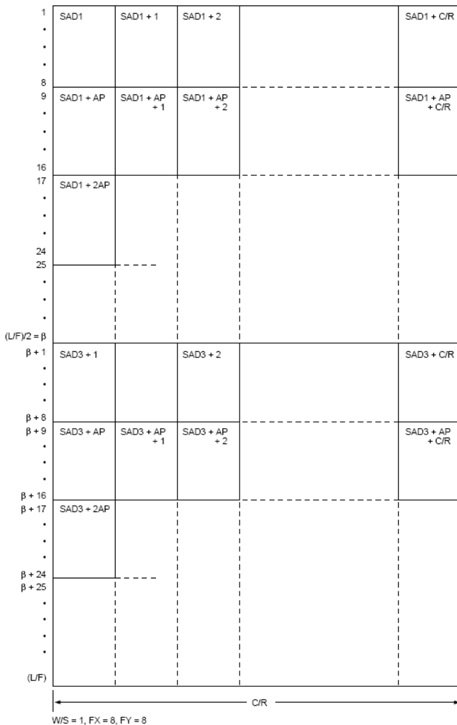
Figure 31. Two-panel display address indexing
