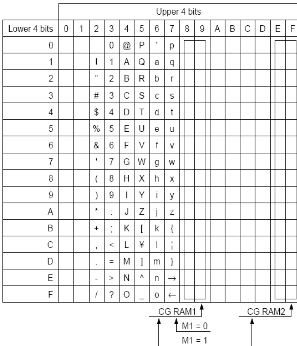
Figure 46. On-chip character codes
