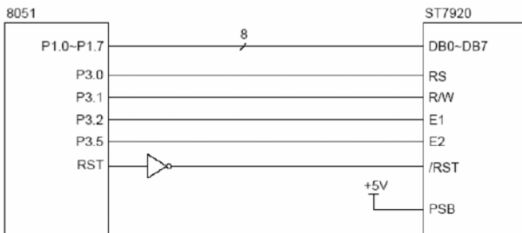
a. Application Circuit 1
