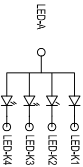
BLU CIRCUIT DIAGRAM
